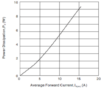
Fig. 1 - Forward Power Dissipation (per diode)
