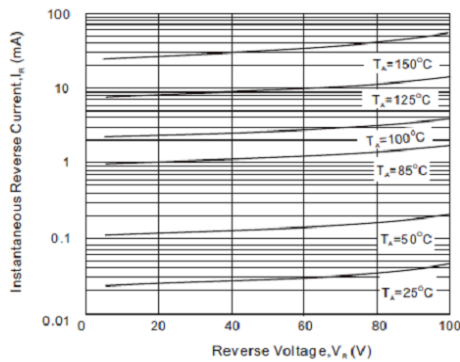
Fig. 3 - Reverse Characteristics (per diode)
