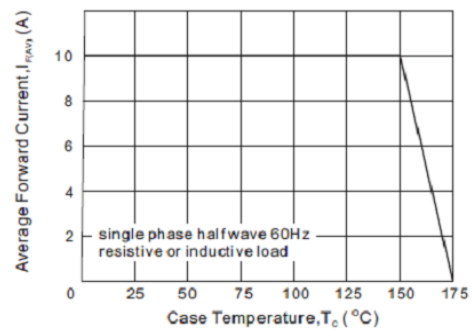
Fig. 4 - Forward Current Derating Curve (per diode)
